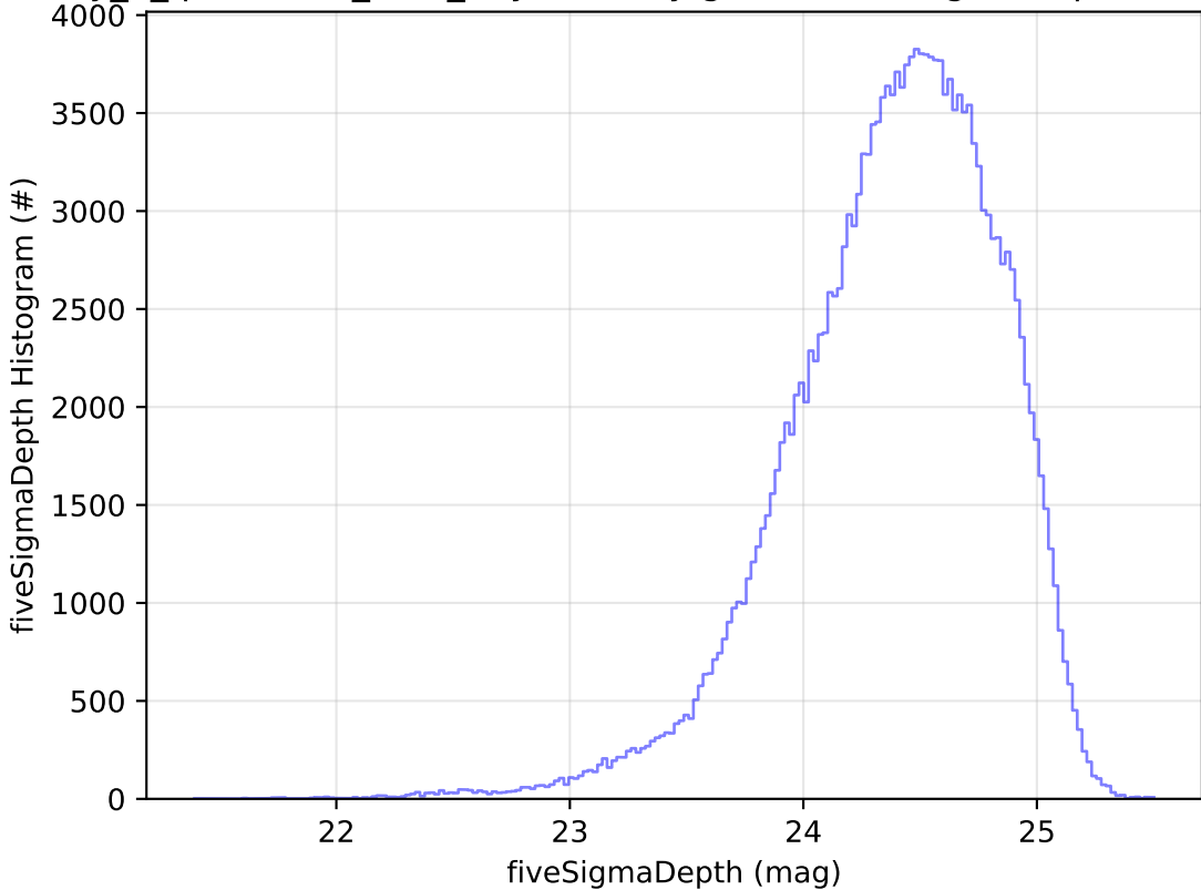
early_u_fpextra3.0_v3.4_10yrs All sky g band: fiveSigmaDepth Histogram
