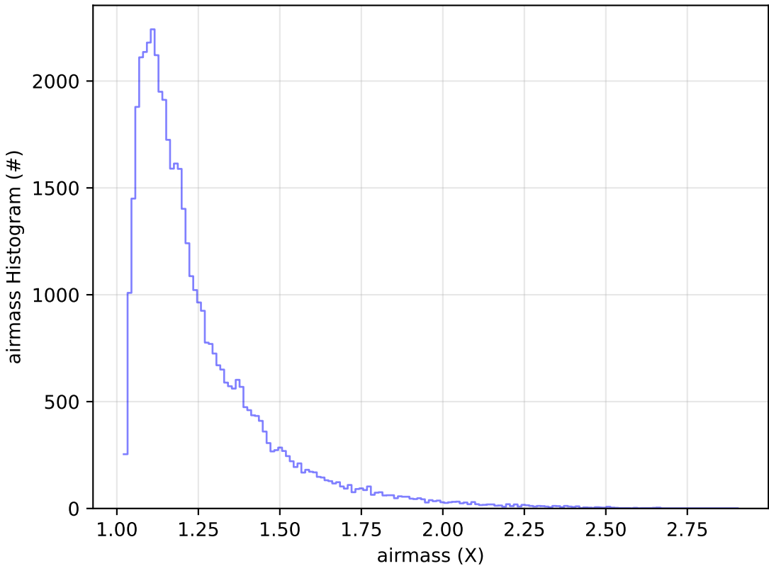
early_u_fpextra3.0_v3.4_10yrs Yr 1 y band: airmass Histogram
