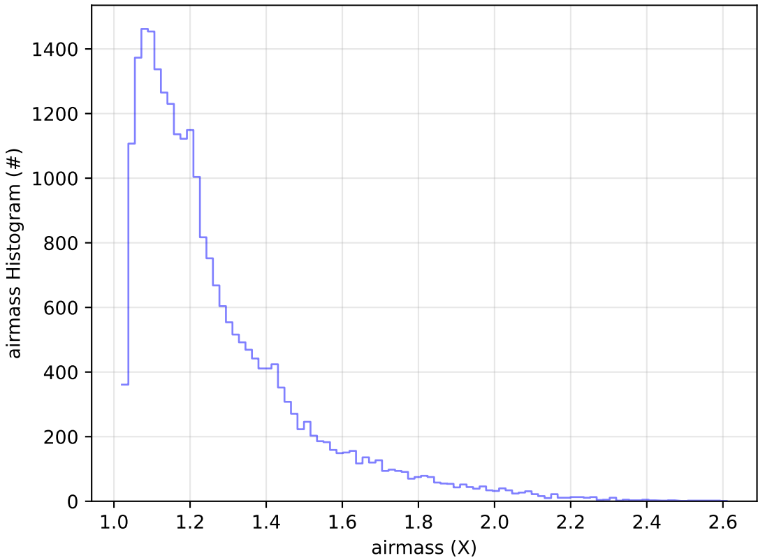
early_u_fpextra3.0_v3.4_10yrs Yr 1 u band: airmass Histogram
