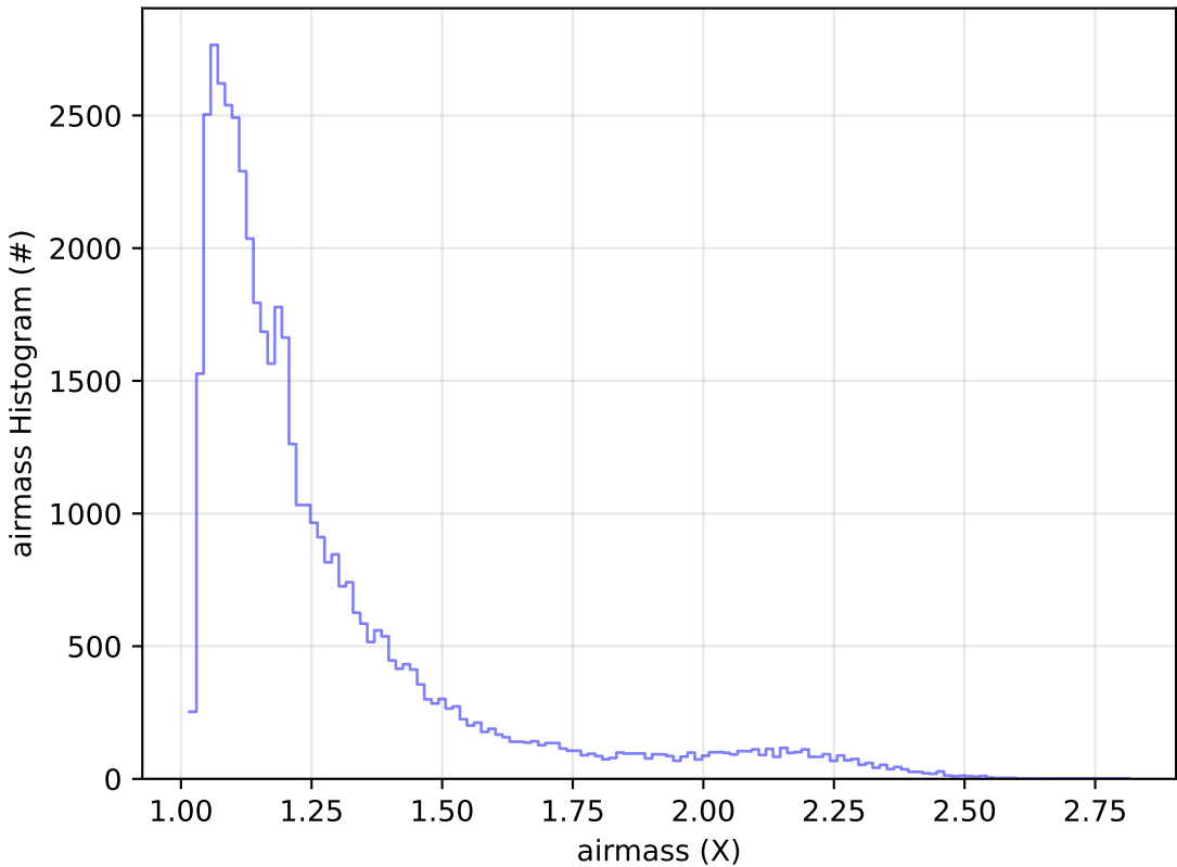
early_u_fpextra3.0_v3.4_10yrs Yr 1 r band: airmass Histogram
