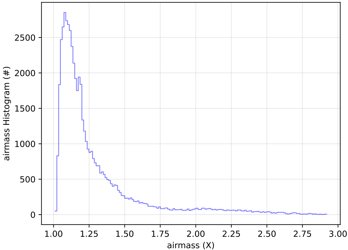
early_u_fpextra3.0_v3.4_10yrs Yr 1 i band: airmass Histogram
