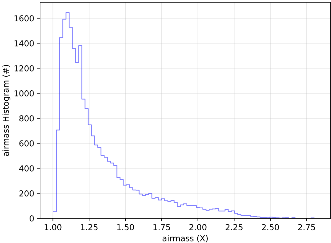
early_u_fpextra3.0_v3.4_10yrs Yr 1 g band: airmass Histogram
