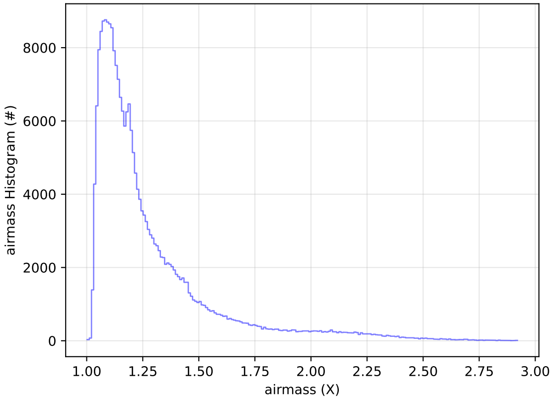
early_u_fpextra3.0_v3.4_10yrs Yr 1 all bands: airmass Histogram
