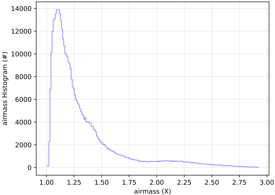
early_u_fpextra3.0_v3.4_10yrs WFD z band: airmass Histogram
