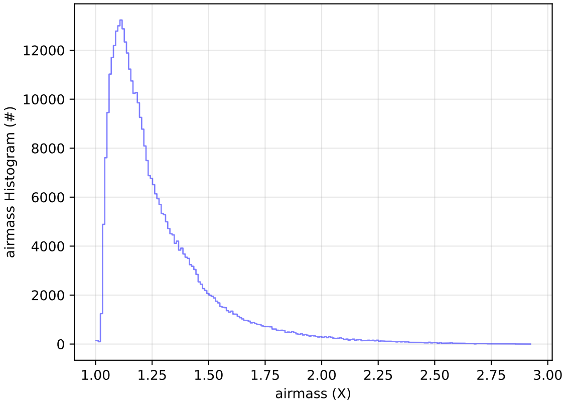
early_u_fpextra3.0_v3.4_10yrs WFD y band: airmass Histogram
