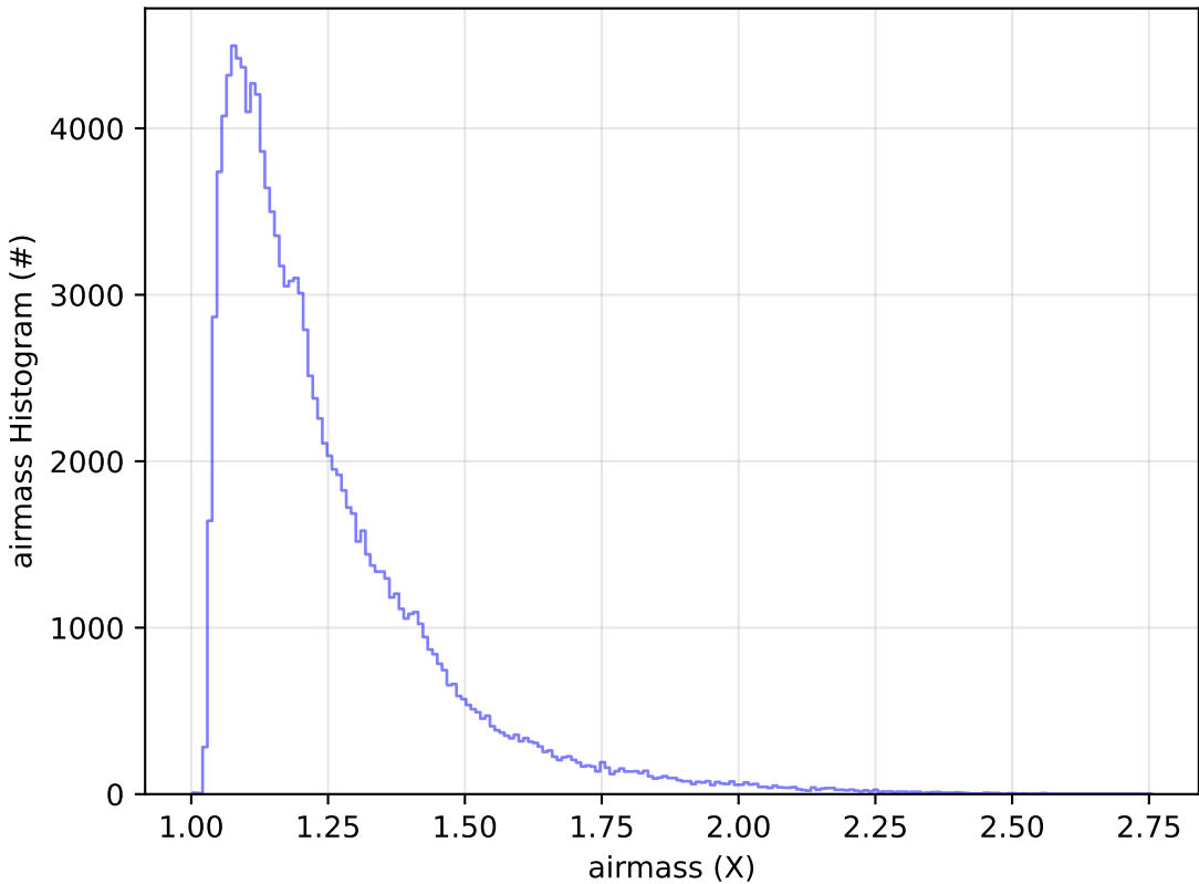
early_u_fpextra3.0_v3.4_10yrs WFD u band: airmass Histogram
