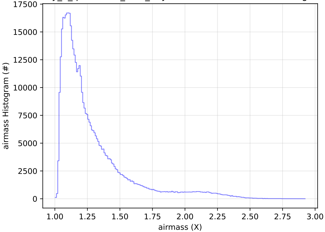
early_u_fpextra3.0_v3.4_10yrs WFD r band: airmass Histogram
