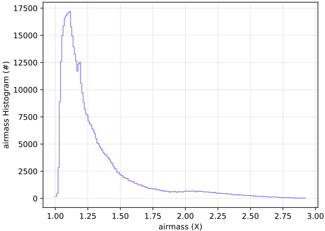
early_u_fpextra3.0_v3.4_10yrs WFD i band: airmass Histogram
