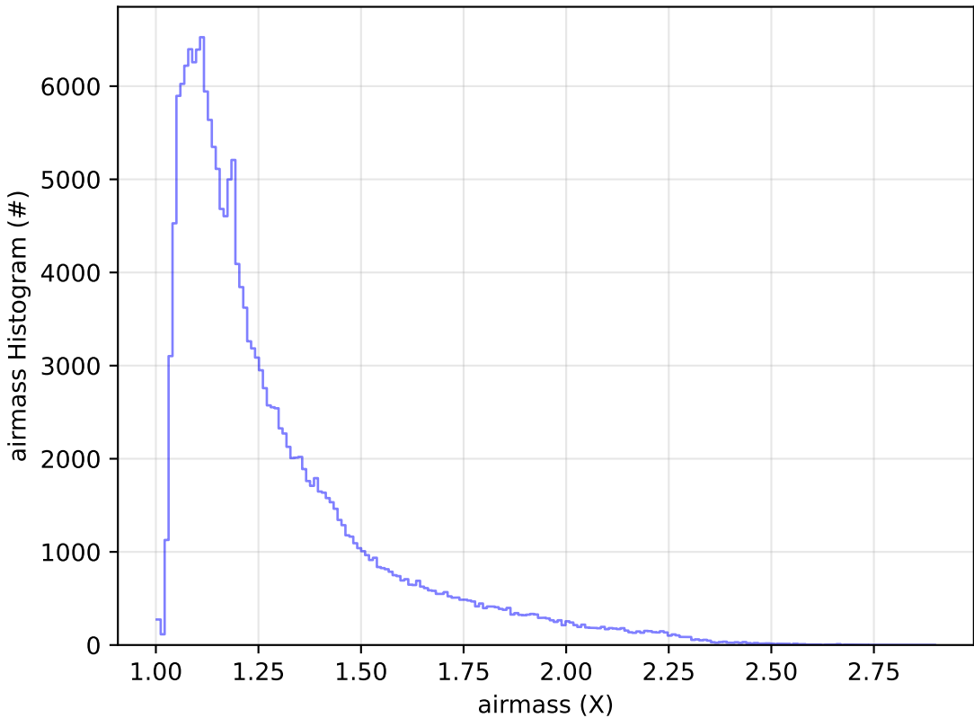
early_u_fpextra3.0_v3.4_10yrs WFD g band: airmass Histogram
