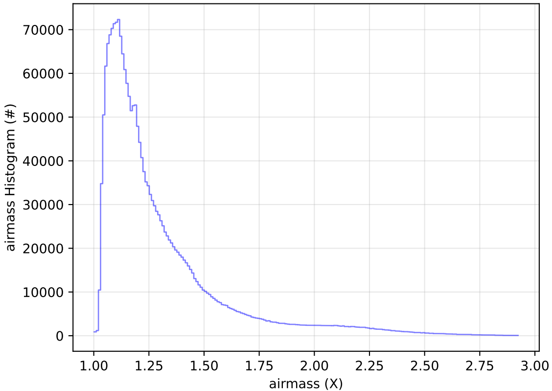
early_u_fpextra3.0_v3.4_10yrs WFD all bands: airmass Histogram
