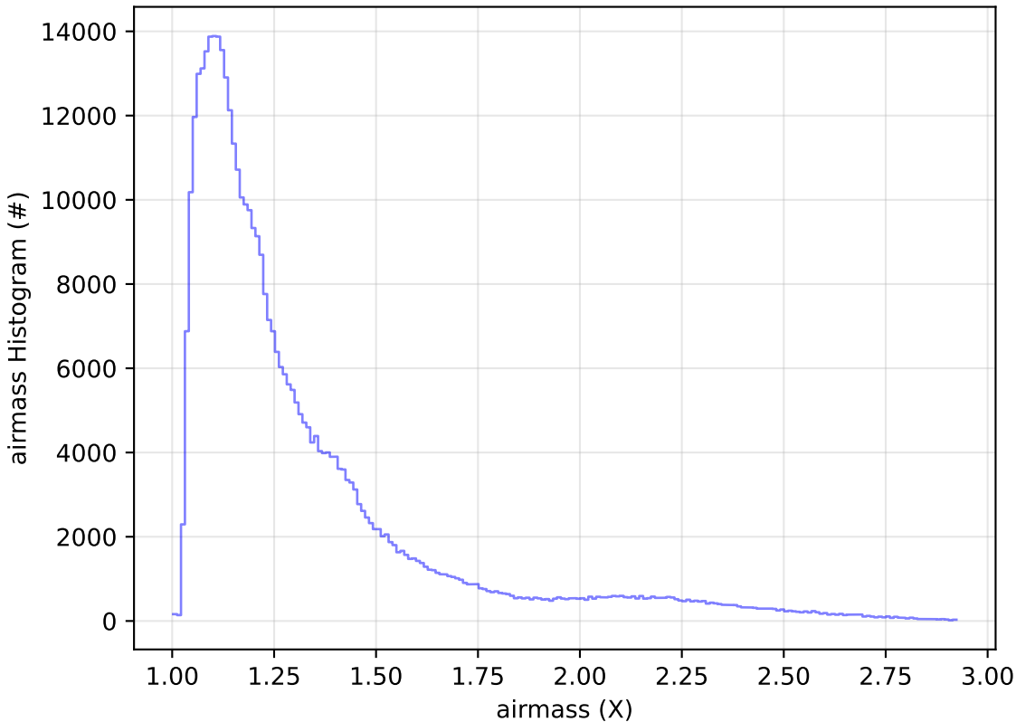
early_u_fpextra3.0_v3.4_10yrs All sky z band: airmass Histogram
