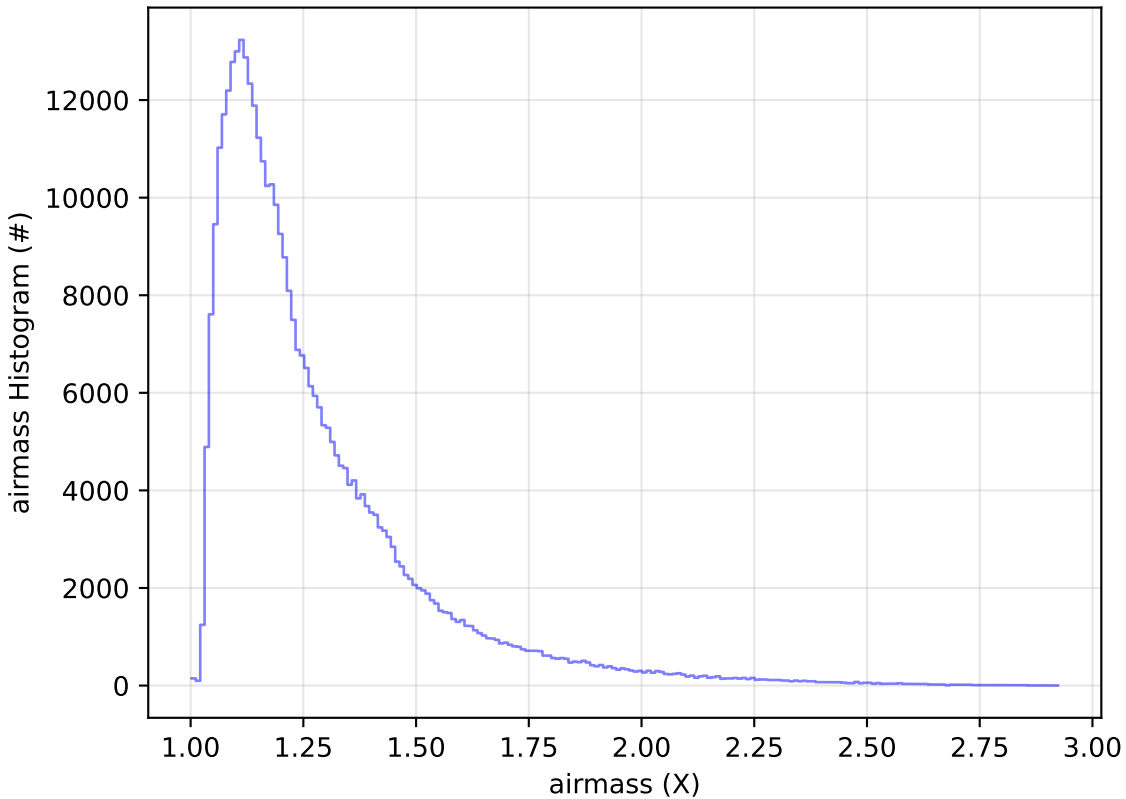
early_u_fpextra3.0_v3.4_10yrs All sky y band: airmass Histogram
