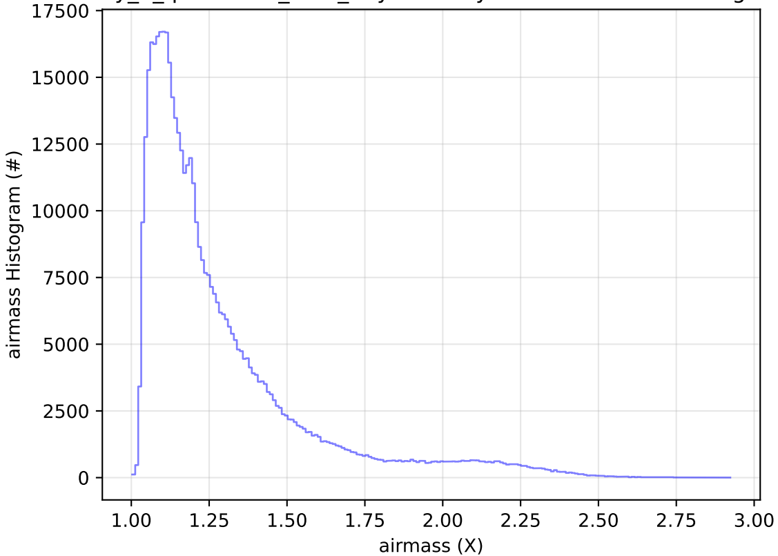
early_u_fpextra3.0_v3.4_10yrs All sky r band: airmass Histogram
