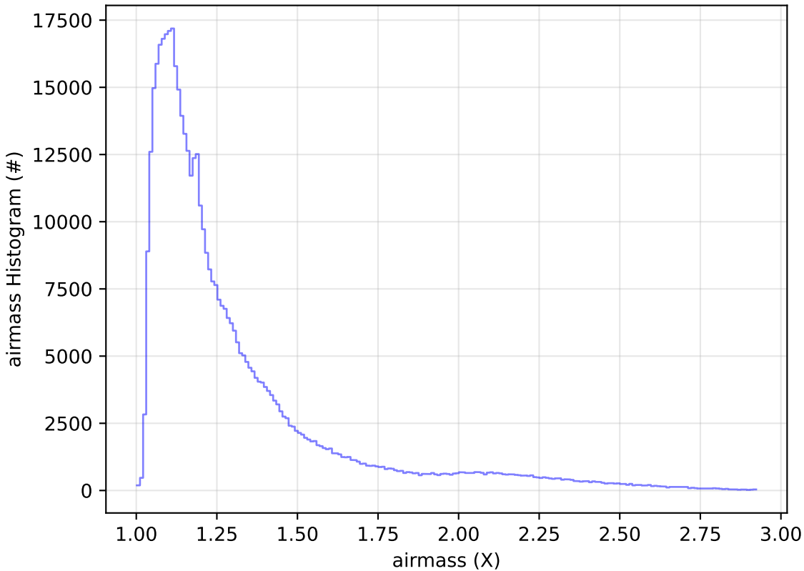
early_u_fpextra3.0_v3.4_10yrs All sky i band: airmass Histogram
