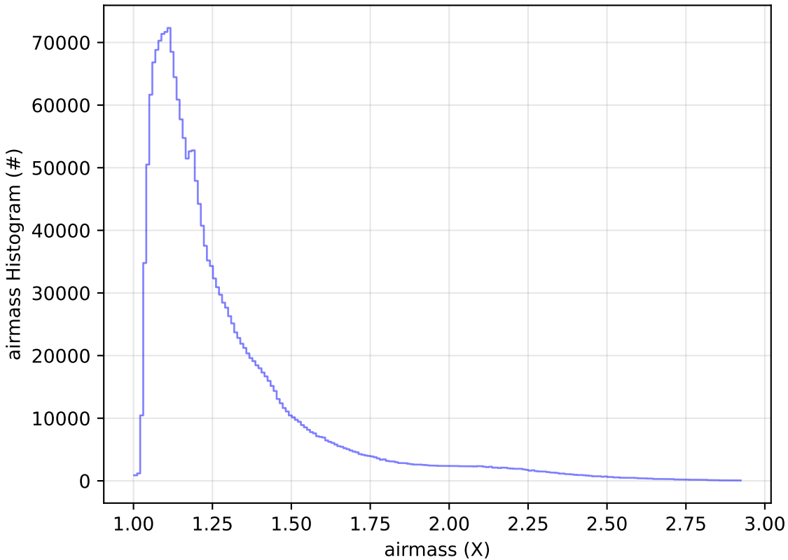
early_u_fpextra3.0_v3.4_10yrs All sky all bands: airmass Histogram
