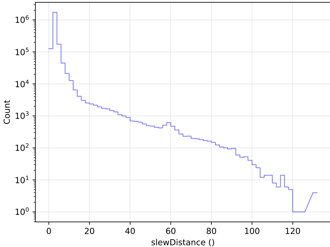
early_u_fpextra3.0_v3.4_10yrs All visits: Slew Distance Histogram
