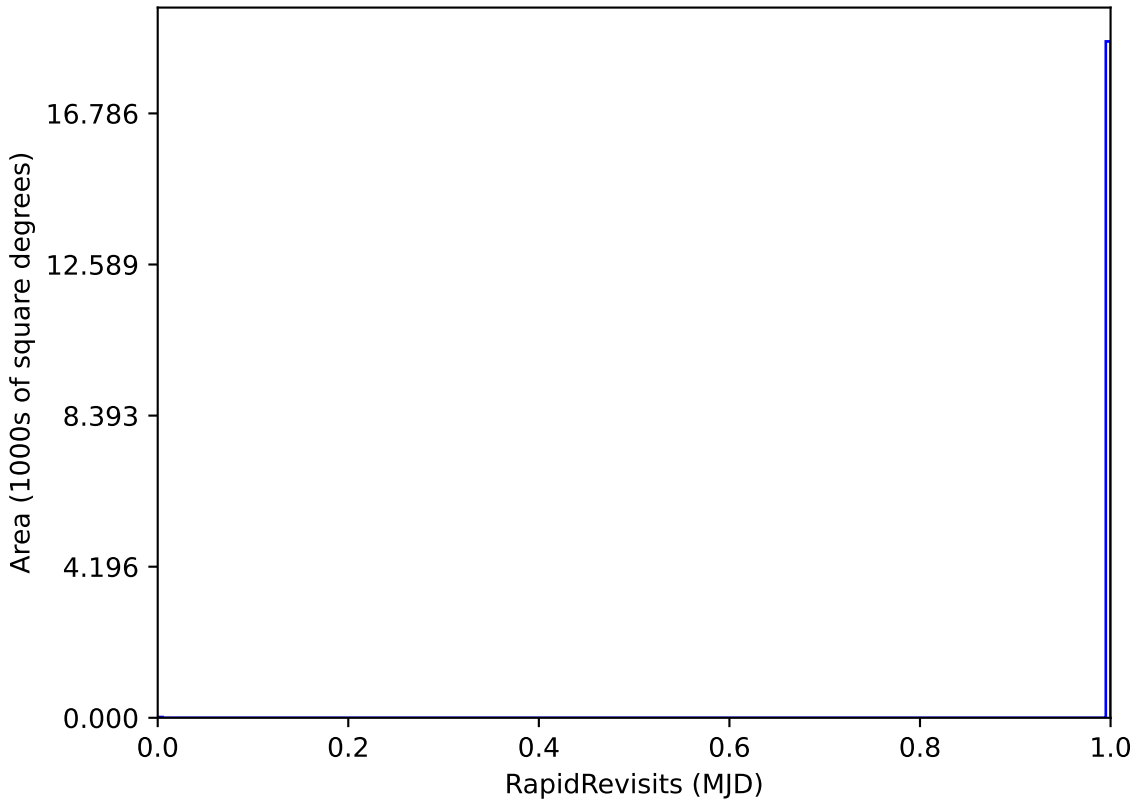
early_u_fpextra3.0_v3.4_10yrs WFD: RapidRevisits
