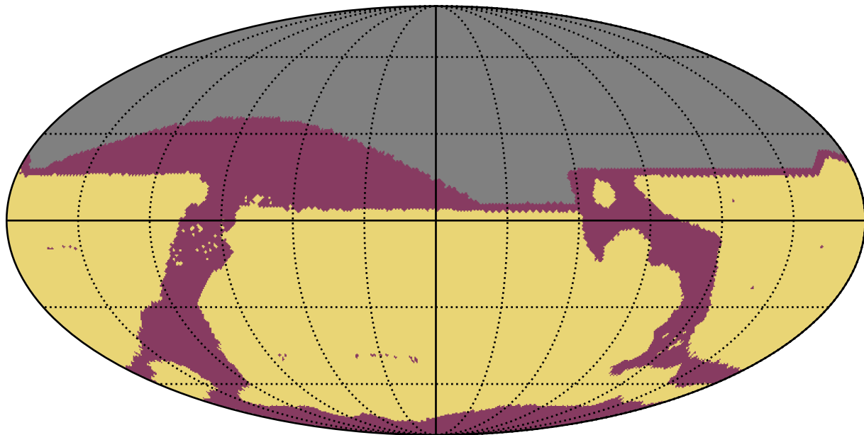
early_u_fpextra3.0_v3.4_10yrs All sky: RapidRevisits
