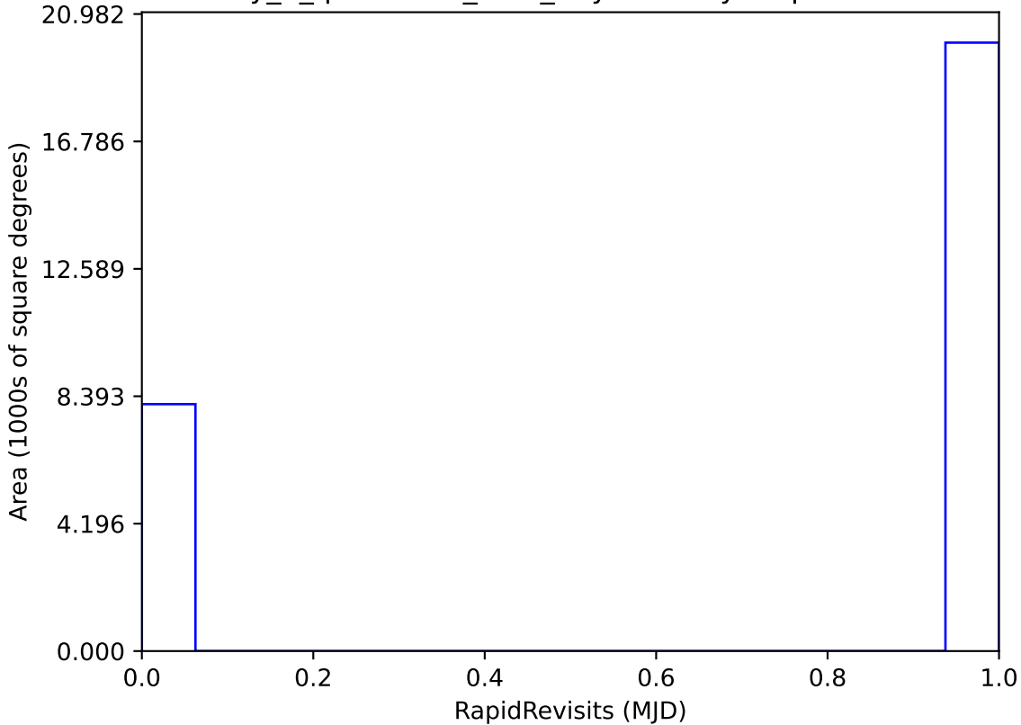
early_u_fpextra3.0_v3.4_10yrs All sky: RapidRevisits
