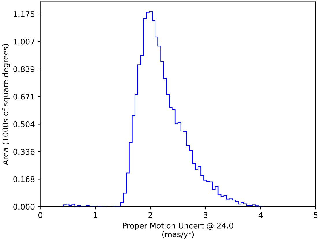
early_u_fpextra3.0_v3.4_10yrs WFD: Proper Motion Uncert @ 24.0
