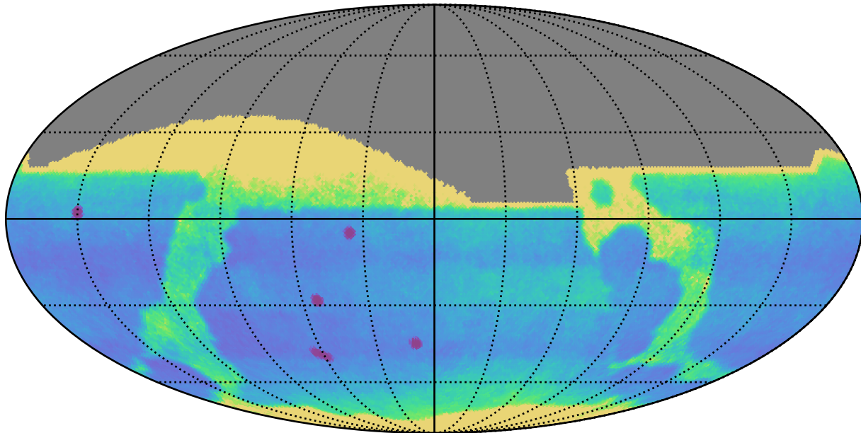
early_u_fpextra3.0_v3.4_10yrs All sky: Proper Motion Uncert @ 24.0
