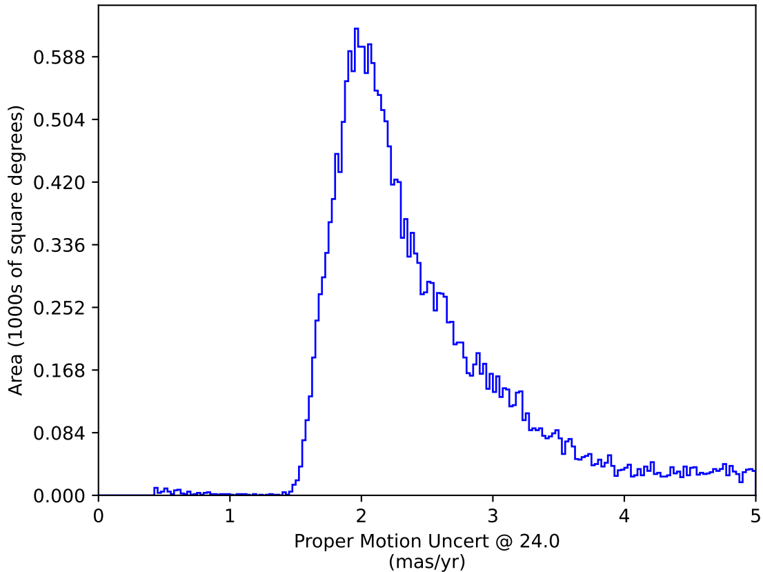
early_u_fpextra3.0_v3.4_10yrs All sky: Proper Motion Uncert @ 24.0
