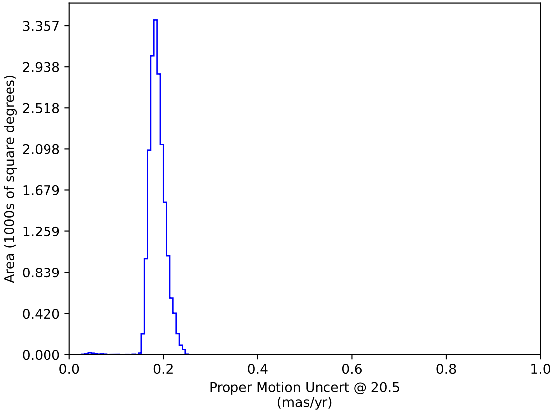
early_u_fpextra3.0_v3.4_10yrs WFD: Proper Motion Uncert @ 20.5
