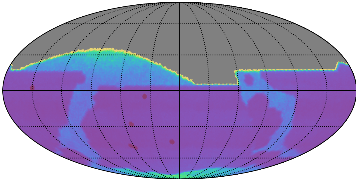
early_u_fpextra3.0_v3.4_10yrs All sky: Proper Motion Uncert @ 20.5
