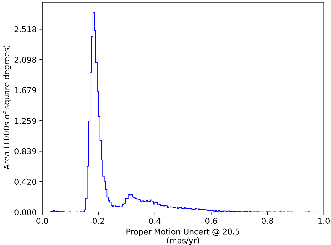
early_u_fpextra3.0_v3.4_10yrs All sky: Proper Motion Uncert @ 20.5
