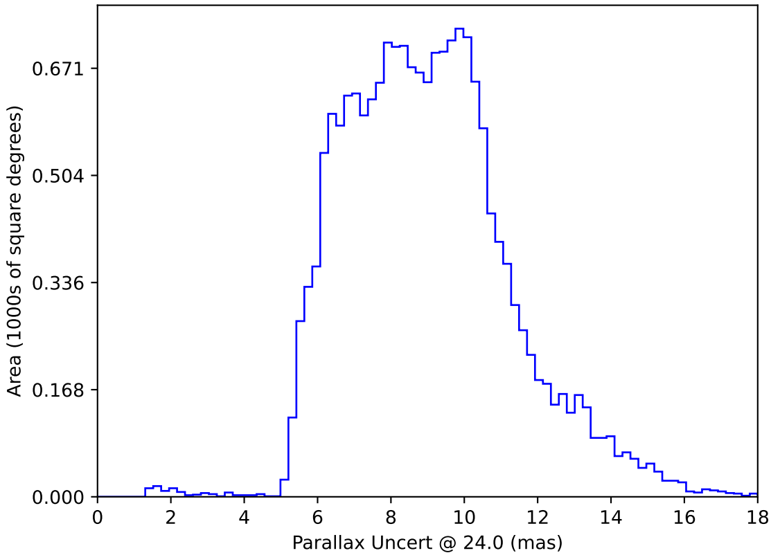
early_u_fpextra3.0_v3.4_10yrs WFD: Parallax Uncert @ 24.0
