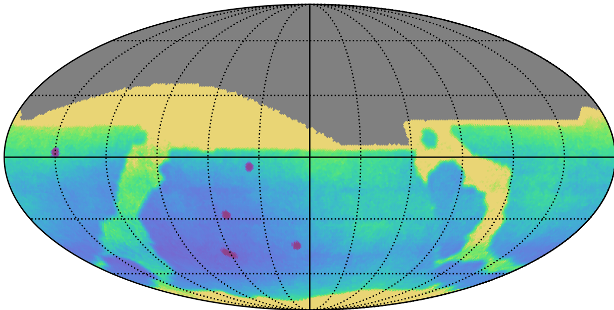
early_u_fpextra3.0_v3.4_10yrs All sky: Parallax Uncert @ 24.0
