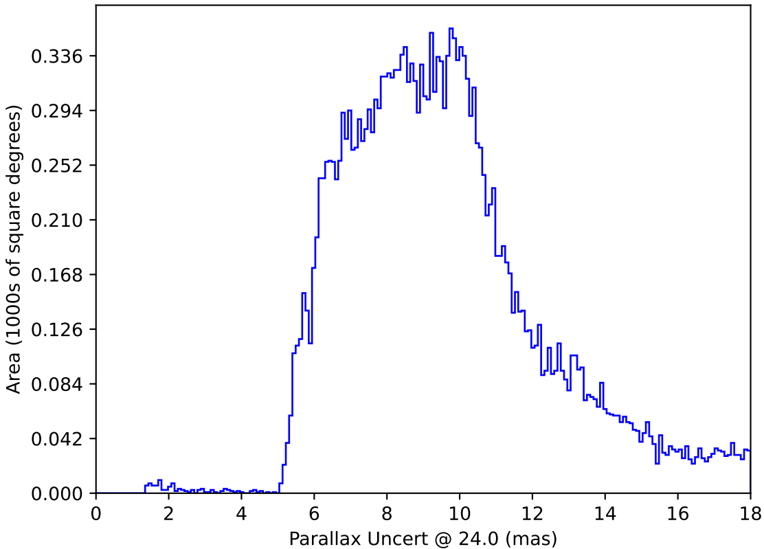
early_u_fpextra3.0_v3.4_10yrs All sky: Parallax Uncert @ 24.0
