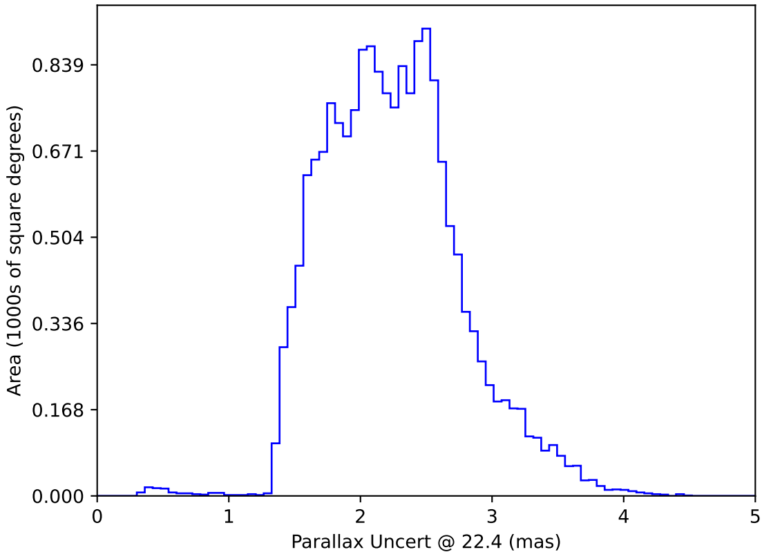
early_u_fpextra3.0_v3.4_10yrs WFD: Parallax Uncert @ 22.4
