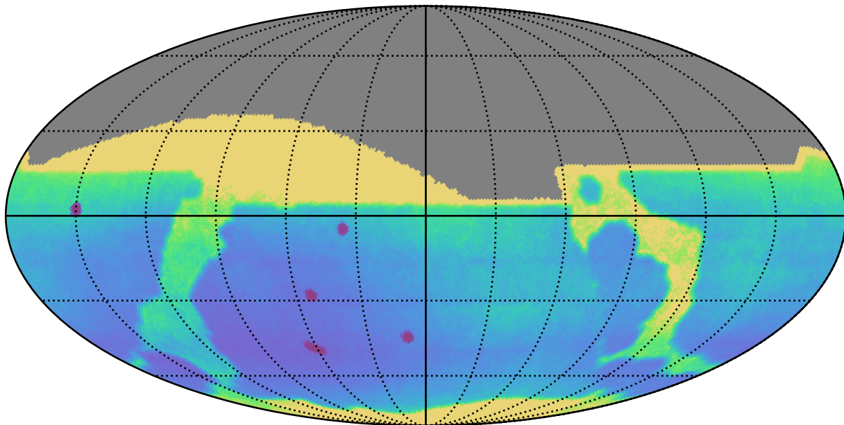
early_u_fpextra3.0_v3.4_10yrs All sky: Parallax Uncert @ 22.4
