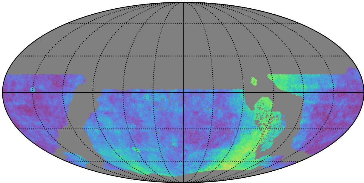
early_u_fpextra3.0_v3.4_10yrs WFD: Parallax Coverage @ 24.0
