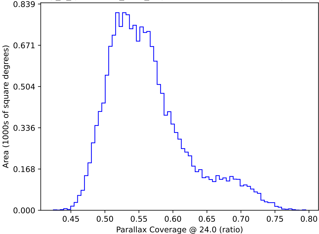
early_u_fpextra3.0_v3.4_10yrs WFD: Parallax Coverage @ 24.0
