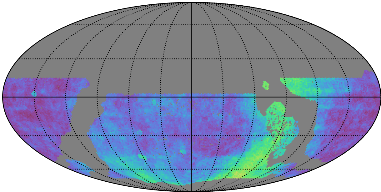
early_u_fpextra3.0_v3.4_10yrs WFD: Parallax Coverage @ 22.4
