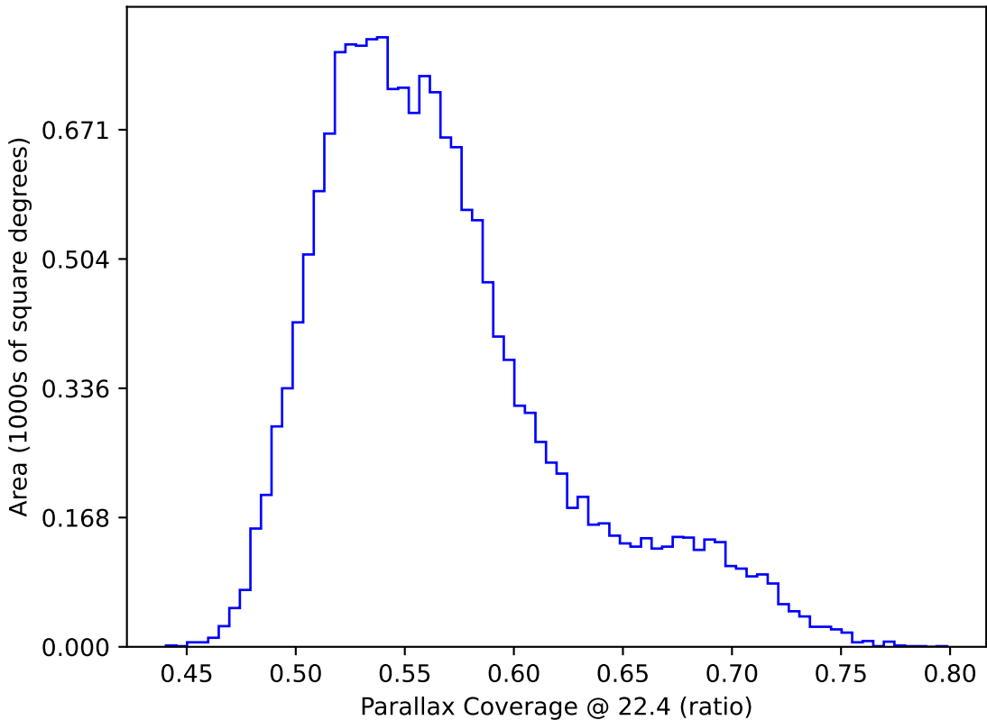
early_u_fpextra3.0_v3.4_10yrs WFD: Parallax Coverage @ 22.4
