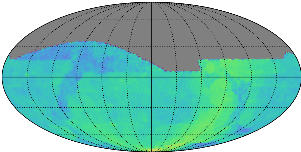
early_u_fpextra3.0_v3.4_10yrs All sky: Parallax Coverage @ 22.4
