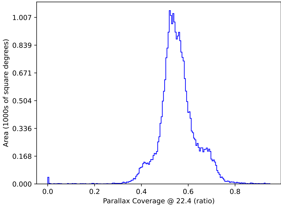
early_u_fpextra3.0_v3.4_10yrs All sky: Parallax Coverage @ 22.4
