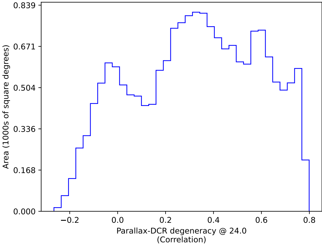
early_u_fpextra3.0_v3.4_10yrs WFD: Parallax-DCR degeneracy @ 24.0
