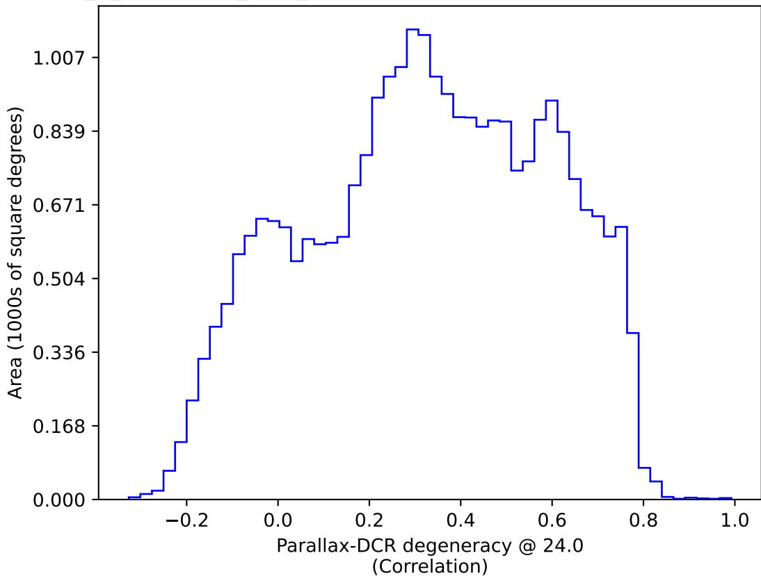
early_u_fpextra3.0_v3.4_10yrs All sky: Parallax-DCR degeneracy @ 24.0
