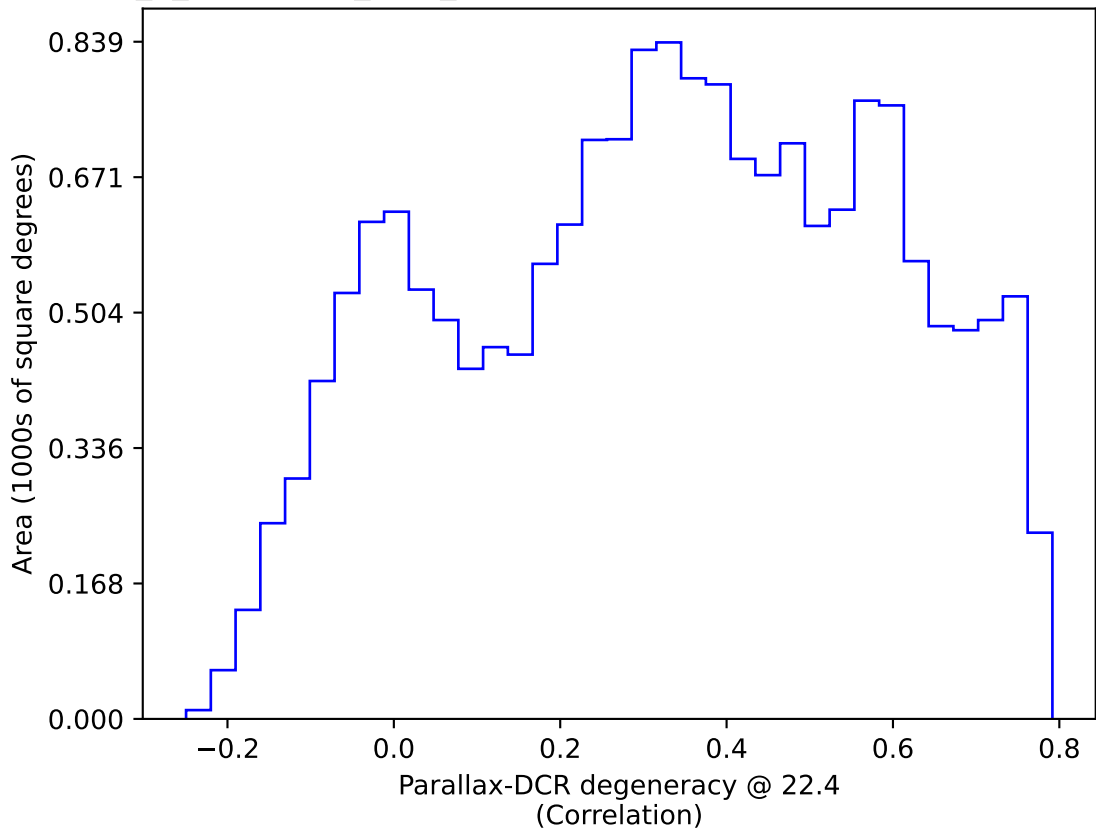
early_u_fpextra3.0_v3.4_10yrs WFD: Parallax-DCR degeneracy @ 22.4
