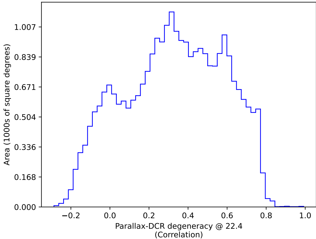
early_u_fpextra3.0_v3.4_10yrs All sky: Parallax-DCR degeneracy @ 22.4
