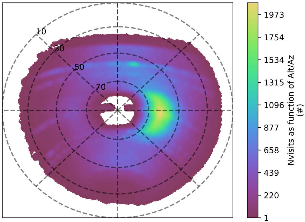
early_u_fpextra3.0_v3.4_10yrs y band: Nvisits as function of Alt/Az
