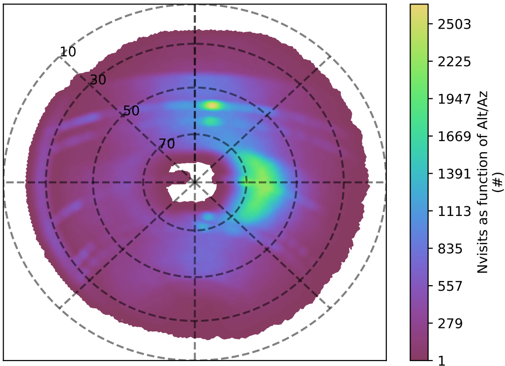
early_u_fpextra3.0_v3.4_10yrs r band: Nvisits as function of Alt/Az
