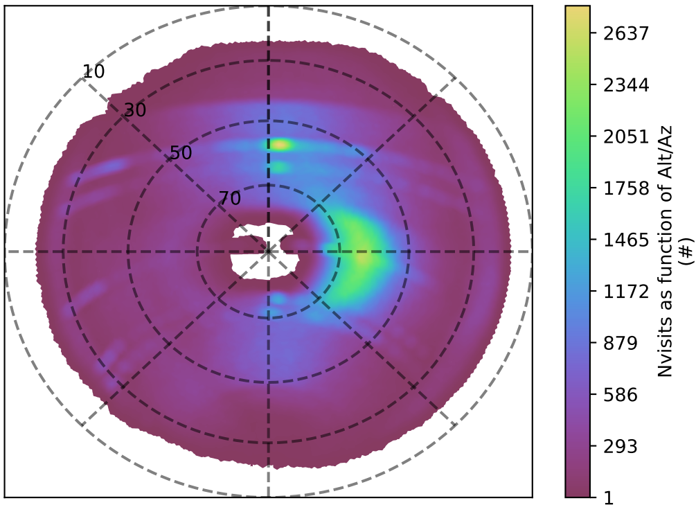
early_u_fpextra3.0_v3.4_10yrs i band: Nvisits as function of Alt/Az
