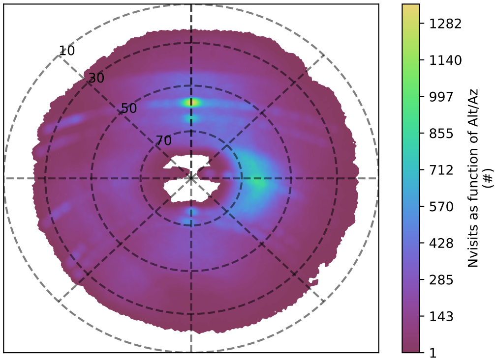
early_u_fpextra3.0_v3.4_10yrs g band: Nvisits as function of Alt/Az
