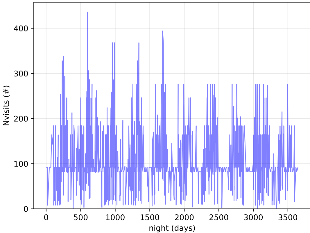
early_u_fpextra3.0_v3.4_10yrs DDF: Nvisits
