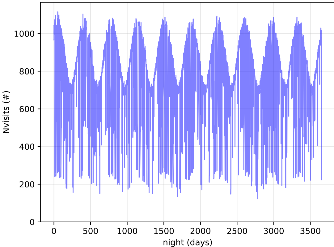
early_u_fpextra3.0_v3.4_10yrs All visits: Nvisits
